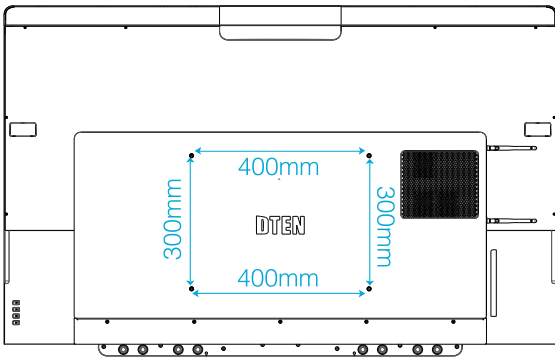
Mounting Hole Pattern: 400 x 300mm
